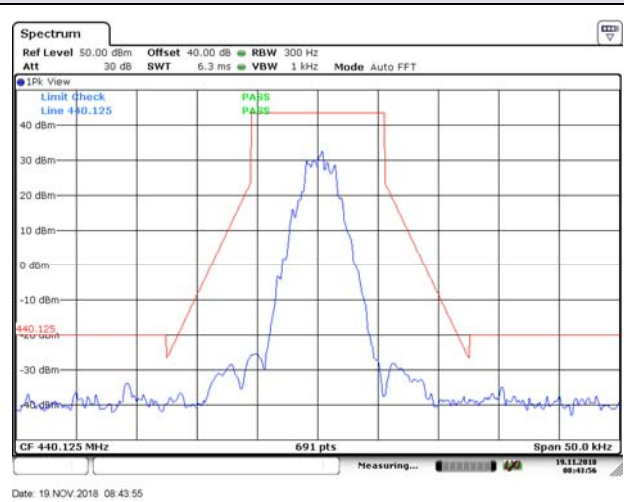
440.125MHz 4FSK
