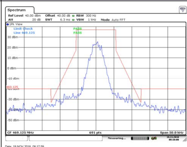
469.125MHz 4FSK
