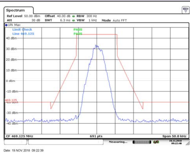
469.125MHz 4FSK
