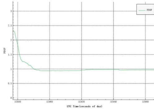
PDOP Value: The Smaller, the Better
