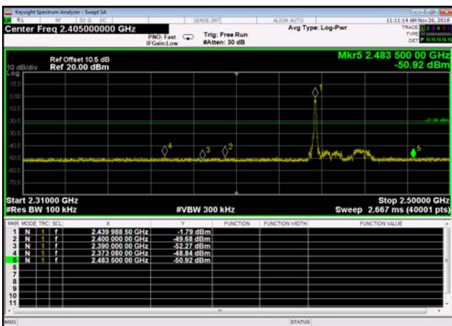
Conducted Emission: 2440 ,Band Edge
