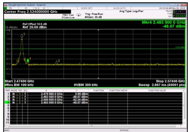
Conducted Emission: 2480 ,Band Edge
