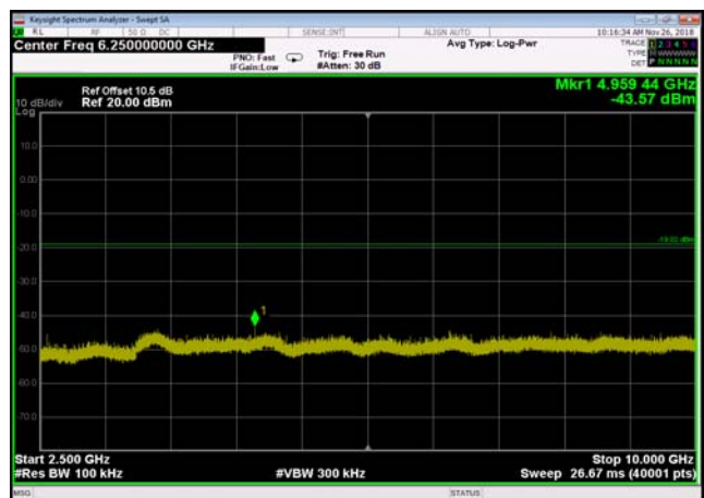
Transmitter Spurious Emission : 2480,2500MHz~10000MHz
